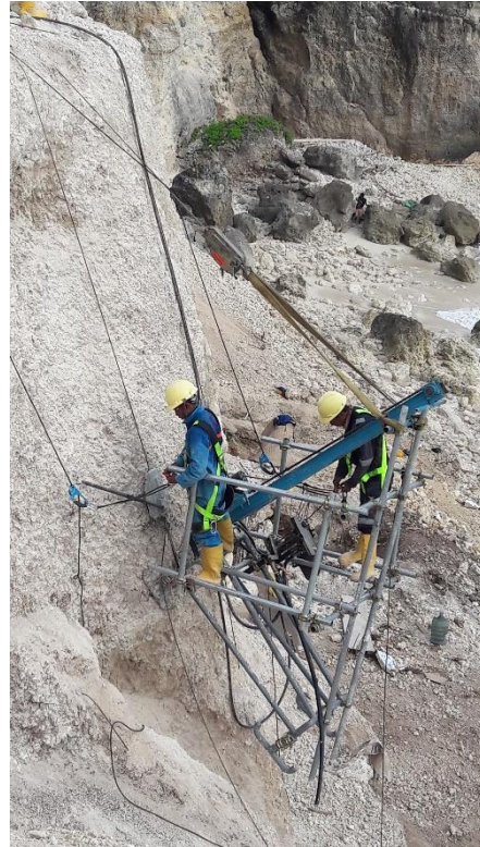
Peralatan Soil Nailing dan Rock Anchor di Lereng
